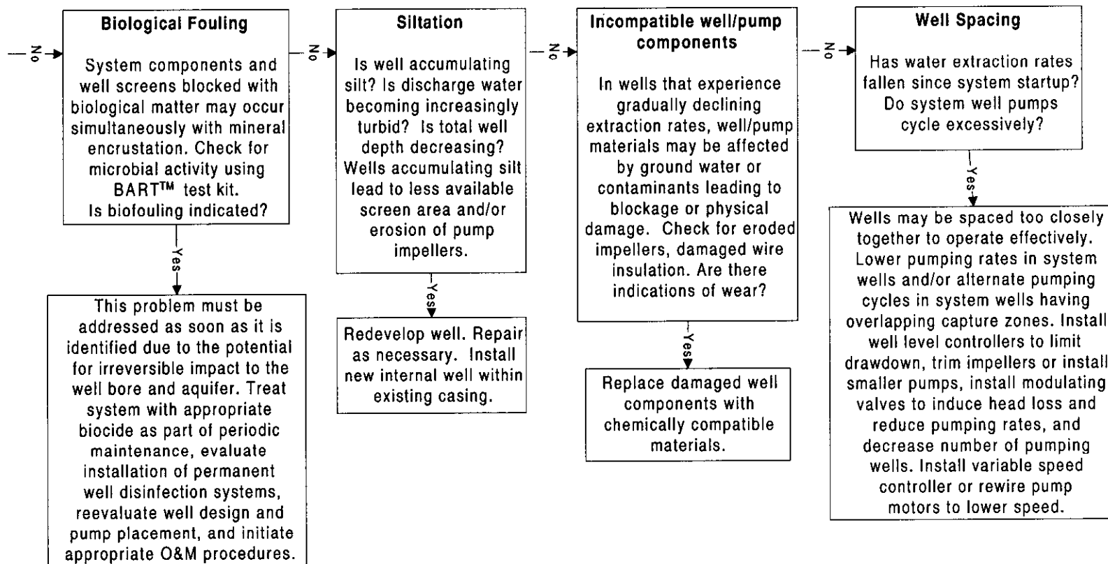
Figure 2-3 Troubleshooting Flow Chart Water Extraction Rate Declining Over Time Sheet 2/2
